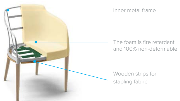
“By Rossetto” moulded polyurethane products Metal frame + cold cure moulding
